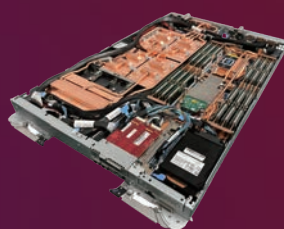
ThinkSystem SD665-N V3
